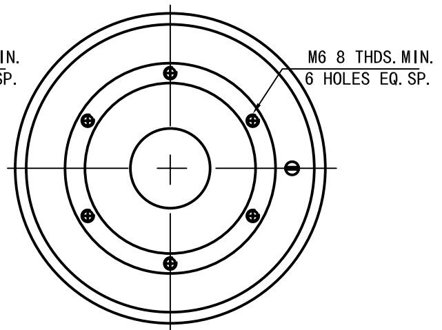
VIEW B
