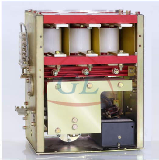
ZK1-630-1.14 (mechanical hold) Vacuum Contactor
