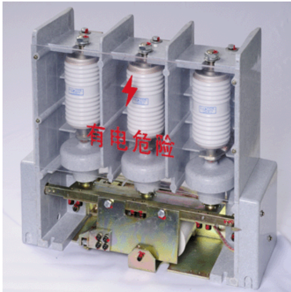
JCZ5-400A/12kV-S AC Vacuum Contactor
