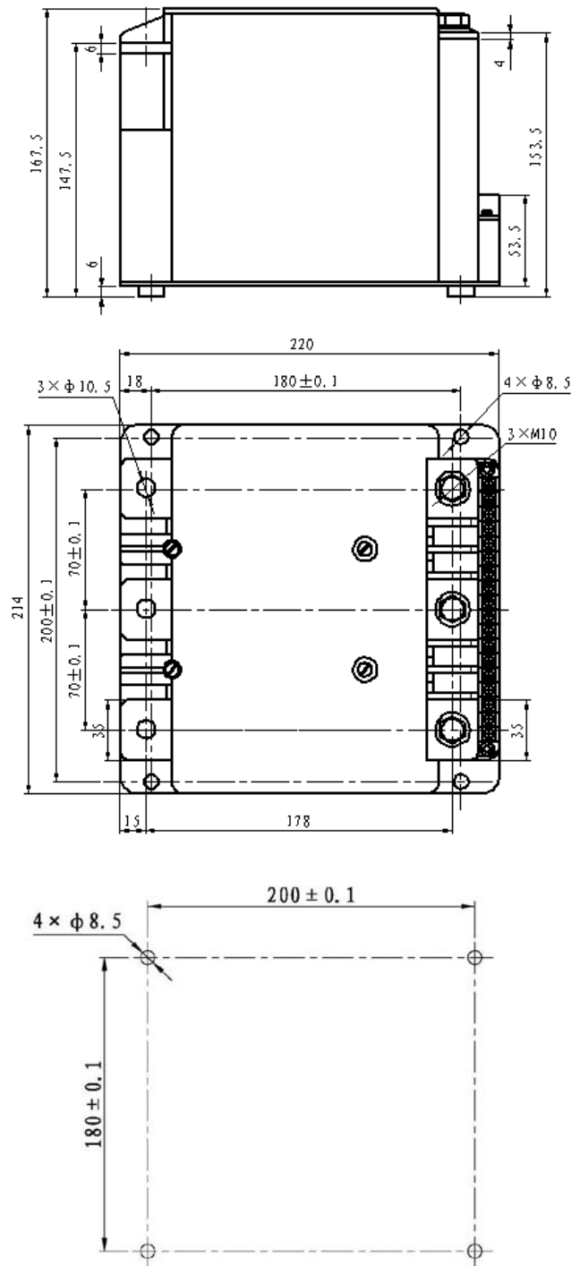
Mounting Dimension
