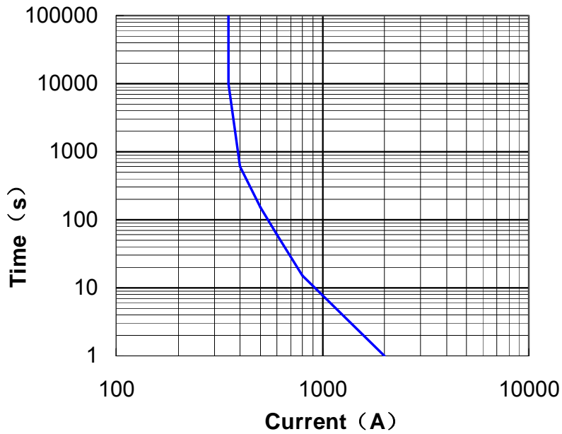
Figure 2. Current Carrying capacity
